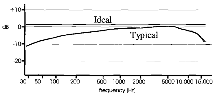
Figure 2: Stylised frequency response curve of a microphone suitable for wildlife sound recording. Ideally, the response curve should be parallel to the horizontal axis. Relatively cheap microphones are more responsive to the frequencies of human speech than other frequencies and so their response curves are not as flat.
